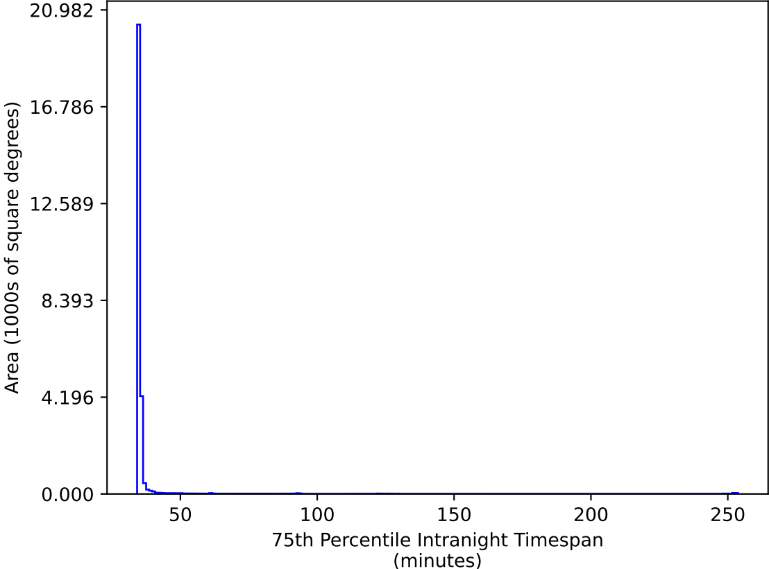
too_elab_2yr_r128_d3_griz_v3.4_10yrs All sky gr bands: 75th Percentile Intranight Timespan
