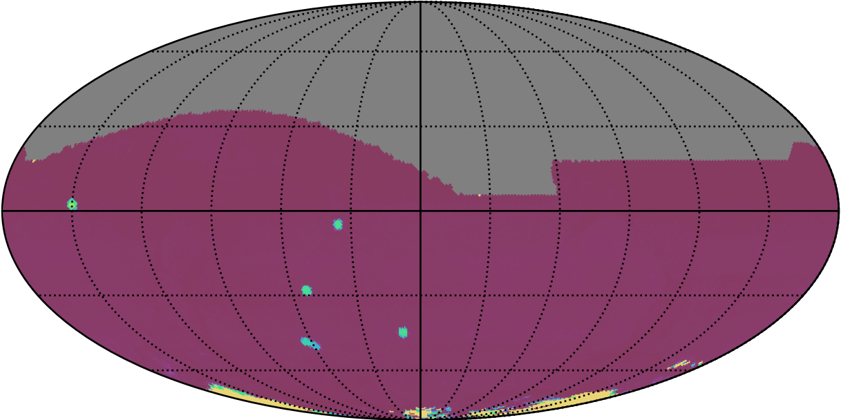
too_elab_2yr_r128_d3_griz_v3.4_10yrs All sky all bands: 75th Percentile Intranight Timespan
