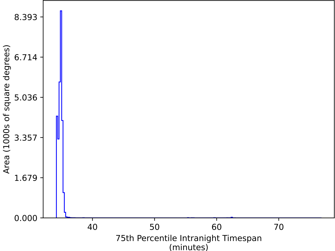
too_elab_2yr_r128_d3_griz_v3.4_10yrs All sky all bands: 75th Percentile Intranight Timespan
