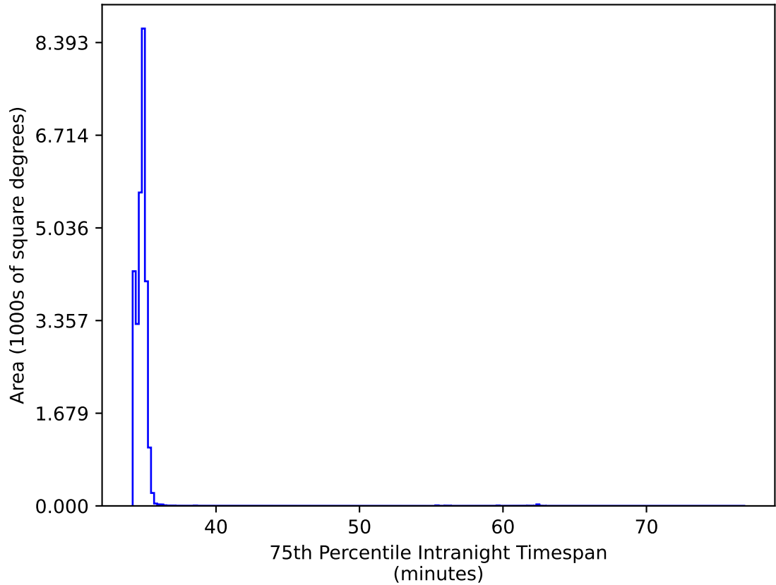
too_elab_2yr_r128_d3_griz_v3.4_10yrs All sky: 75th Percentile Intranight Timespan
