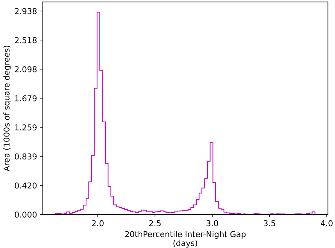
too_elab_2yr_r128_d3_griz_v3.4_10yrs WFD z band: 20thPercentile Inter-Night Gap
