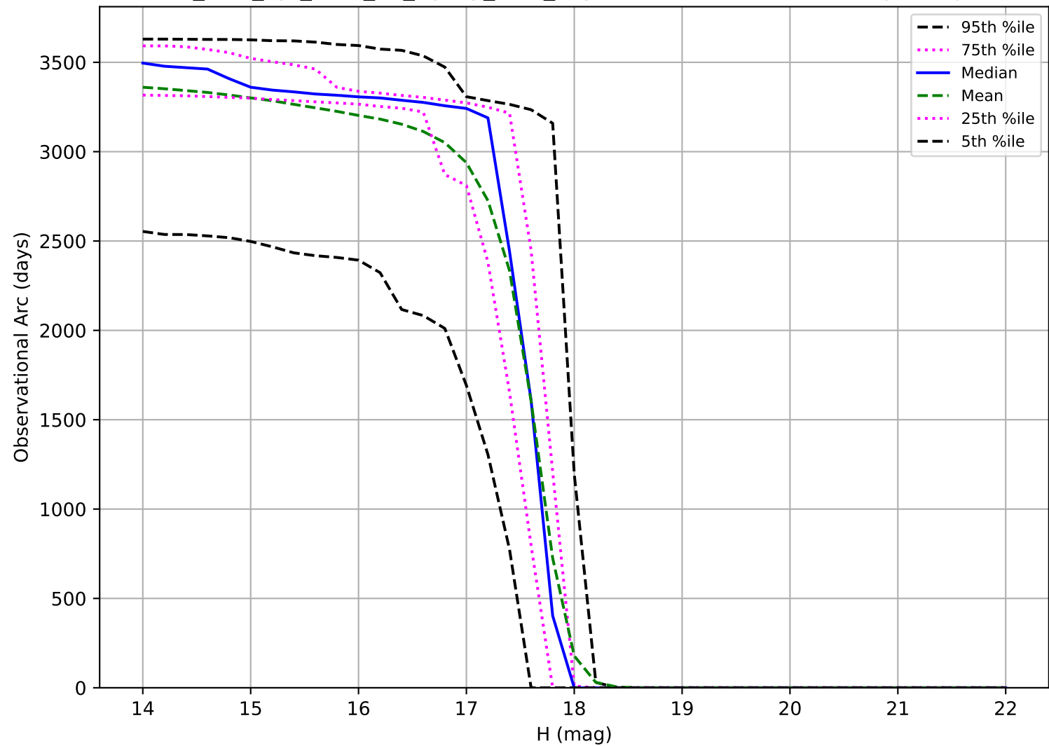
too_elab_2yr_r128_d2_ugrizy_v3.4_10yrs: Observational Arc Length Trojan
