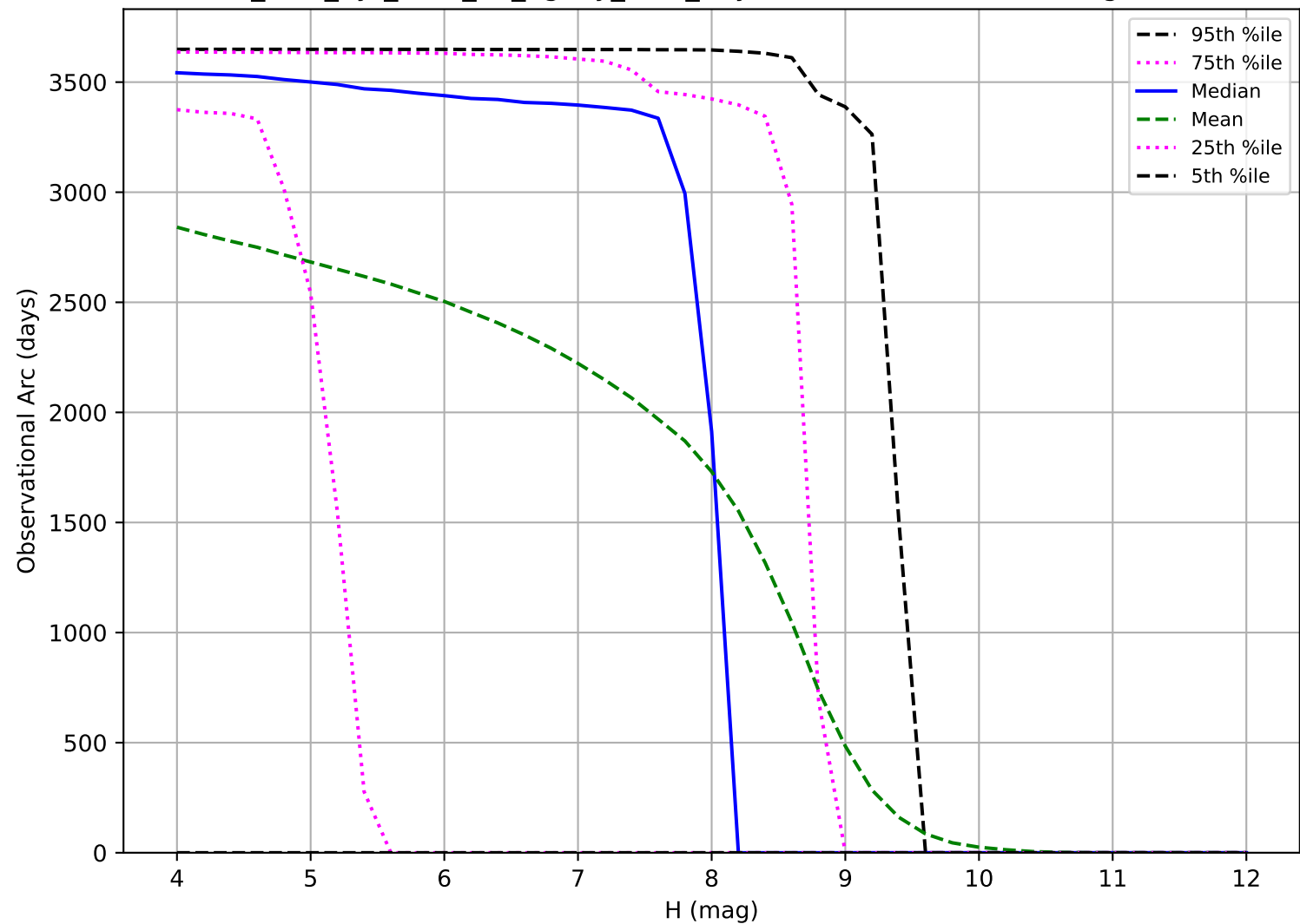
too_elab_2yr_r128_d2_ugrizy_v3.4_10yrs: Observational Arc Length TNO
