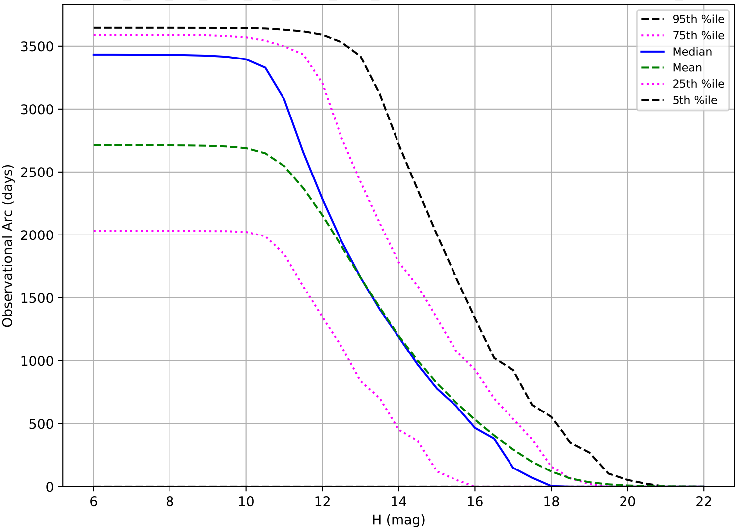
too_elab_2yr_r128_d2_ugrizy_v3.4_10yrs: Observational Arc Length OCC_r5
