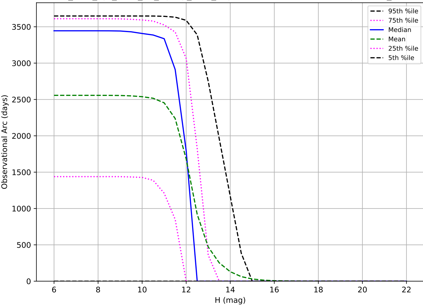
too_elab_2yr_r128_d2_ugrizy_v3.4_10yrs: Observational Arc Length OCC_r20
