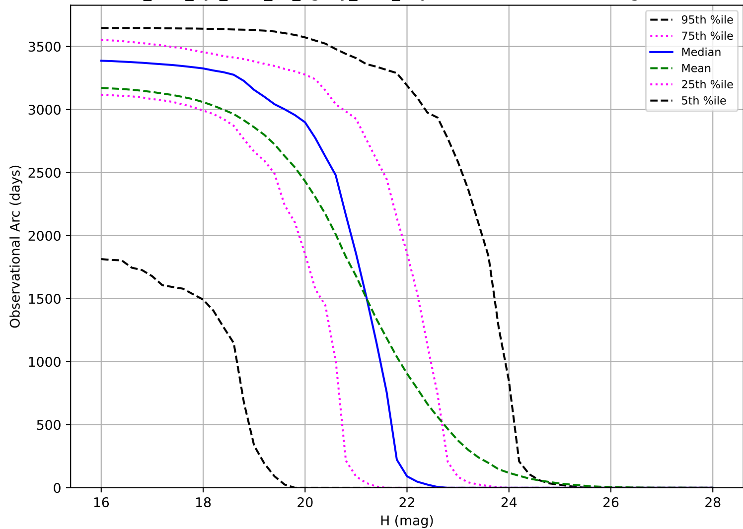
too_elab_2yr_r128_d2_ugrizy_v3.4_10yrs: Observational Arc Length NEO
