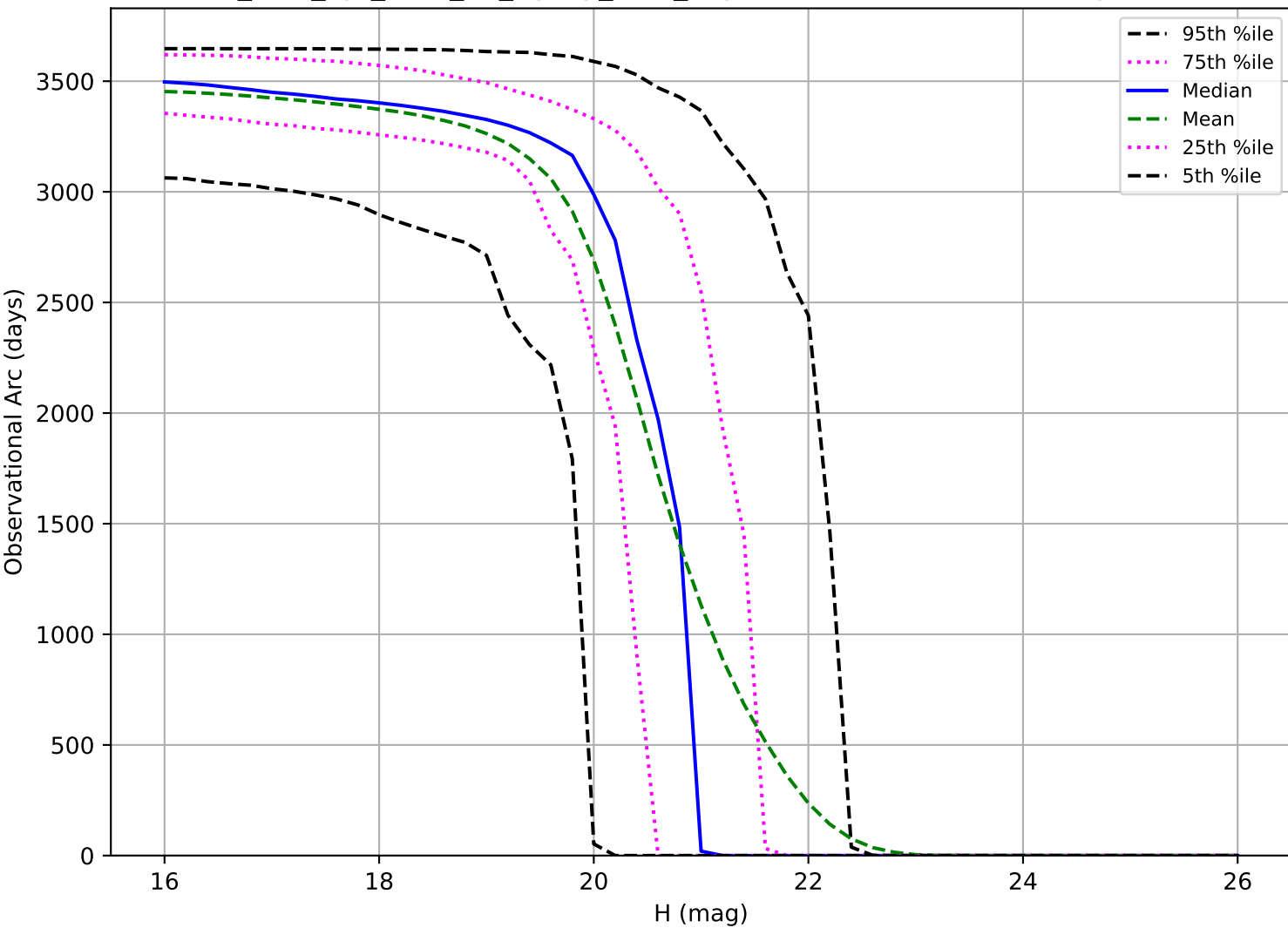
too_elab_2yr_r128_d2_ugrizy_v3.4_10yrs: Observational Arc Length MBA
