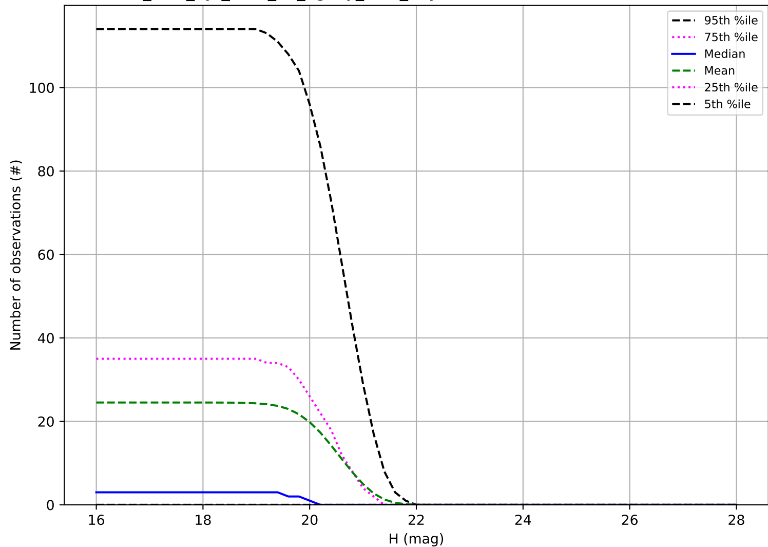
too_elab_2yr_r128_d2_ugrizy_v3.4_10yrs: Number of observations Vatira
