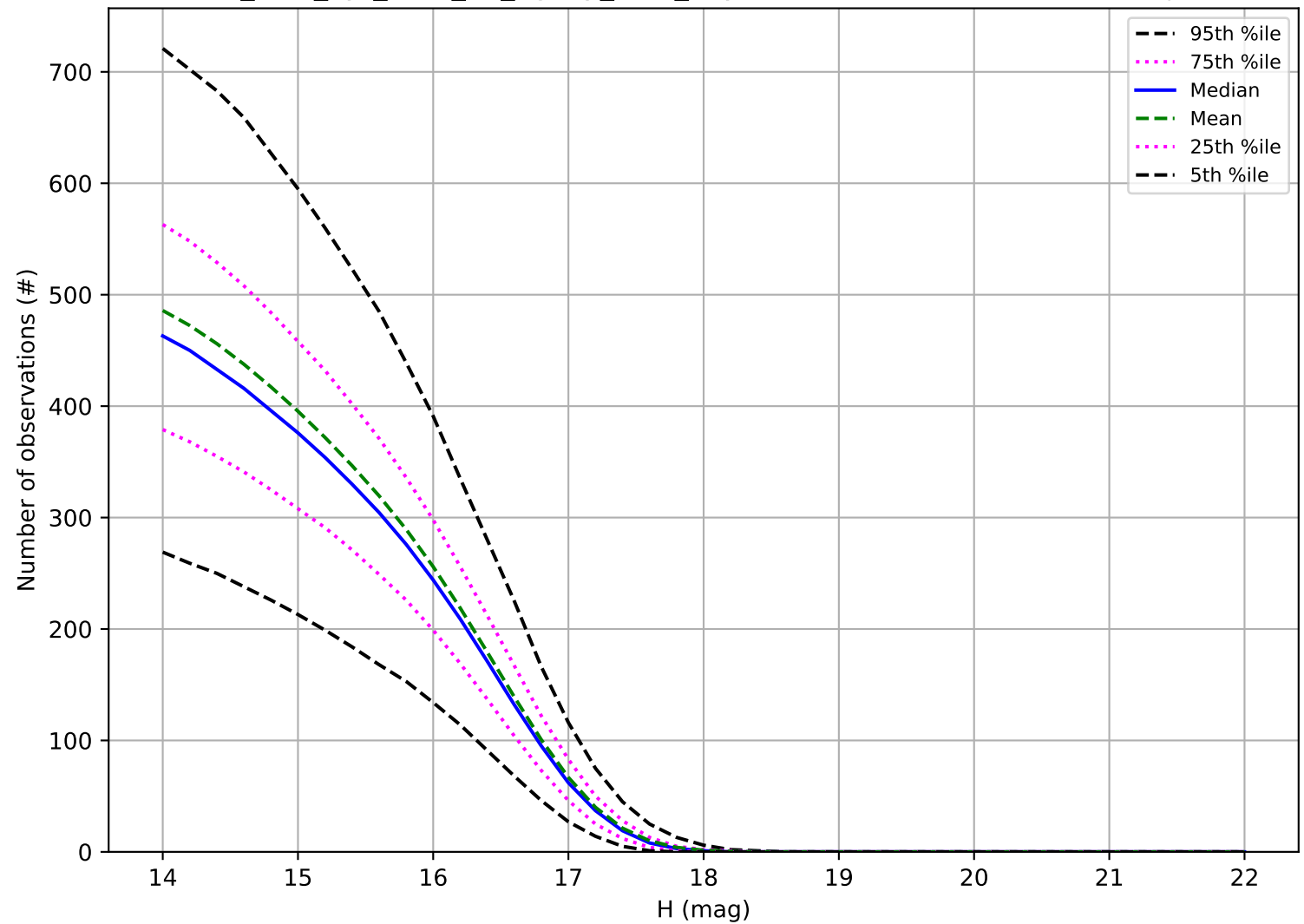
too_elab_2yr_r128_d2_ugrizy_v3.4_10yrs: Number of observations Trojan
