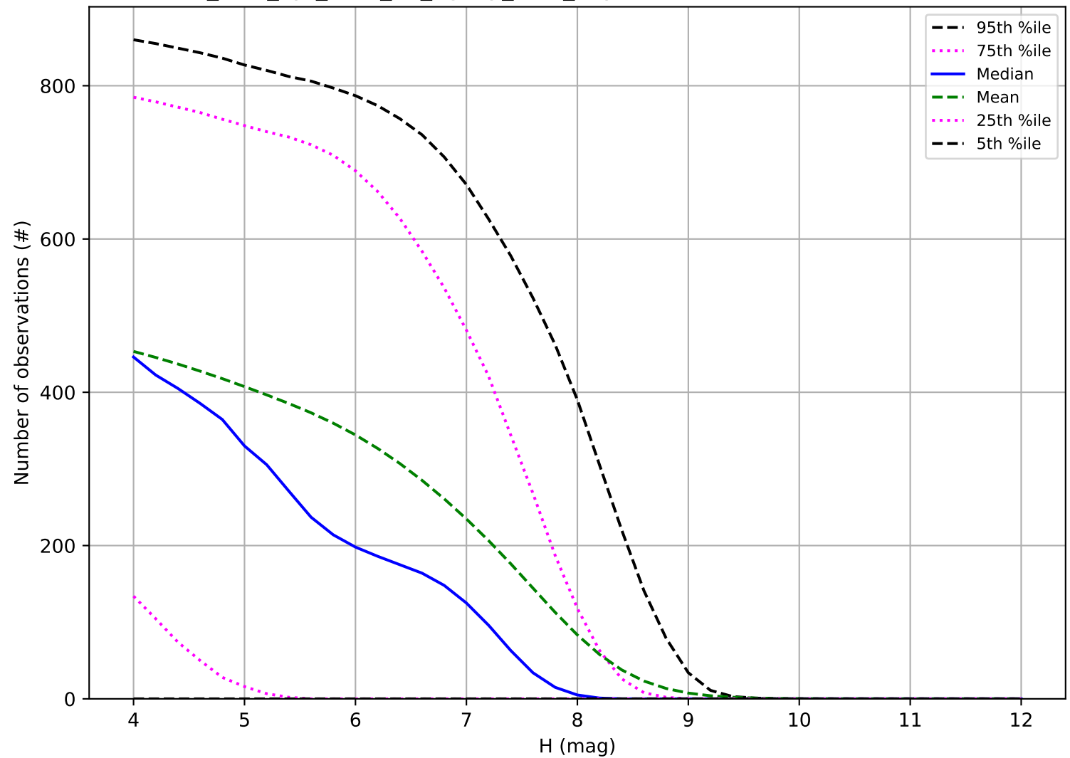
too_elab_2yr_r128_d2_ugrizy_v3.4_10yrs: Number of observations TNO
