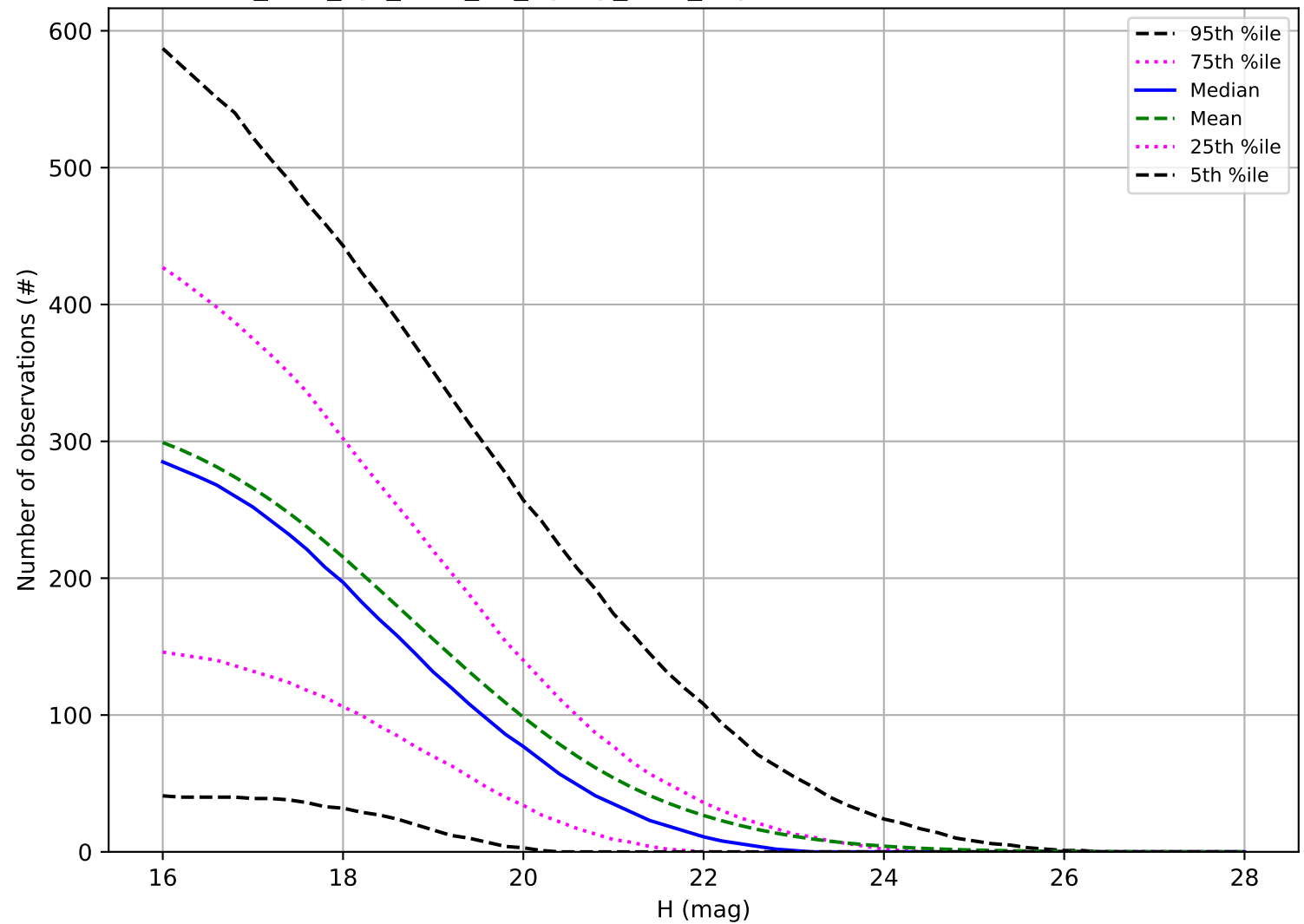
too_elab_2yr_r128_d2_ugrizy_v3.4_10yrs: Number of observations PHA
