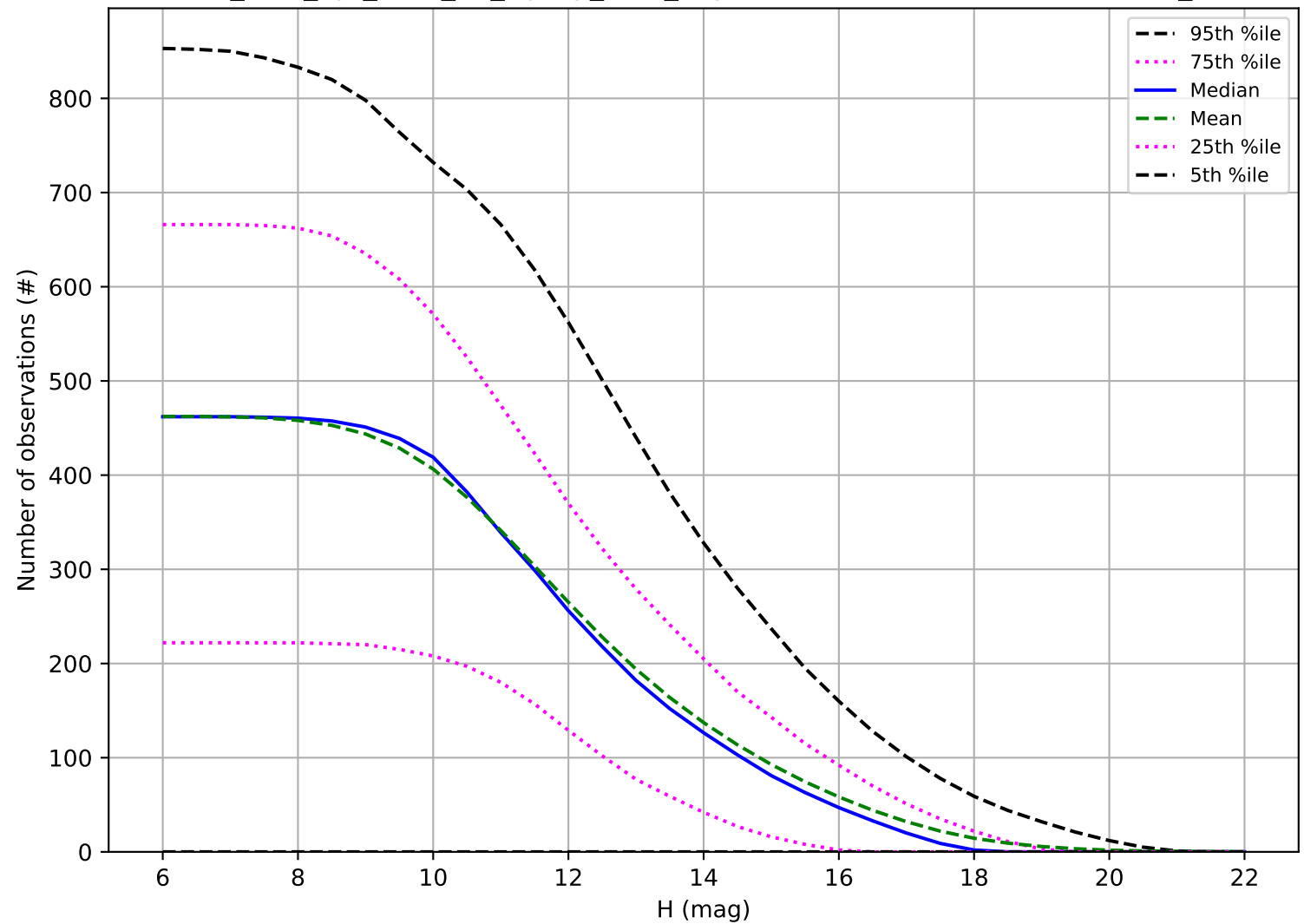
too_elab_2yr_r128_d2_ugrizy_v3.4_10yrs: Number of observations OCC_r5
