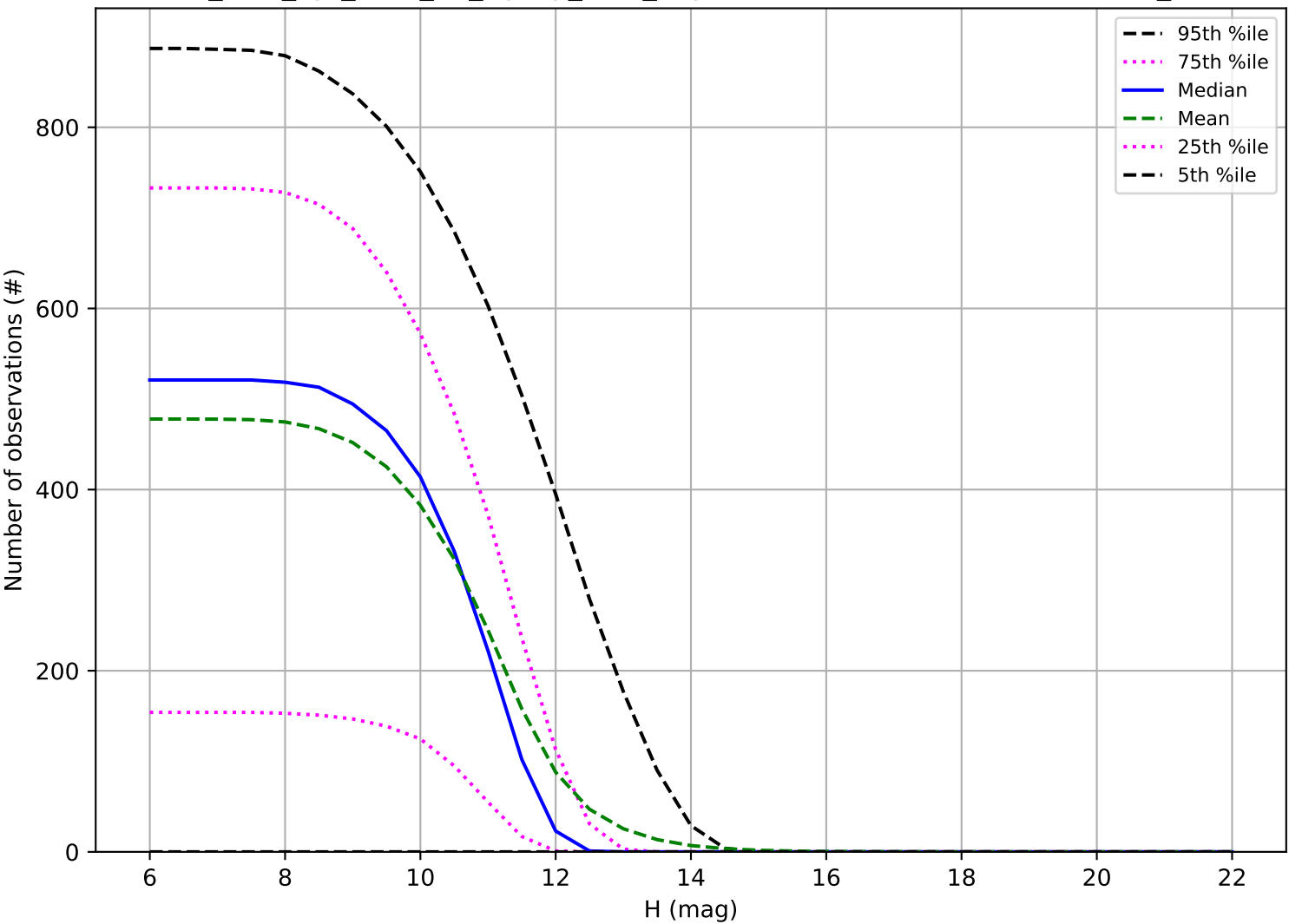
too_elab_2yr_r128_d2_ugrizy_v3.4_10yrs: Number of observations OCC_r20
