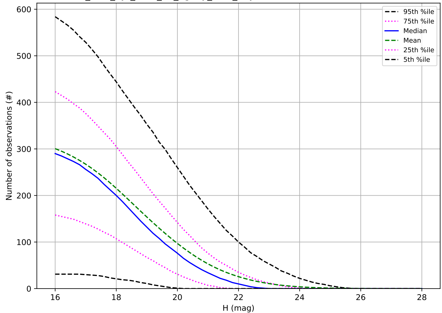
too_elab_2yr_r128_d2_ugrizy_v3.4_10yrs: Number of observations NEO
