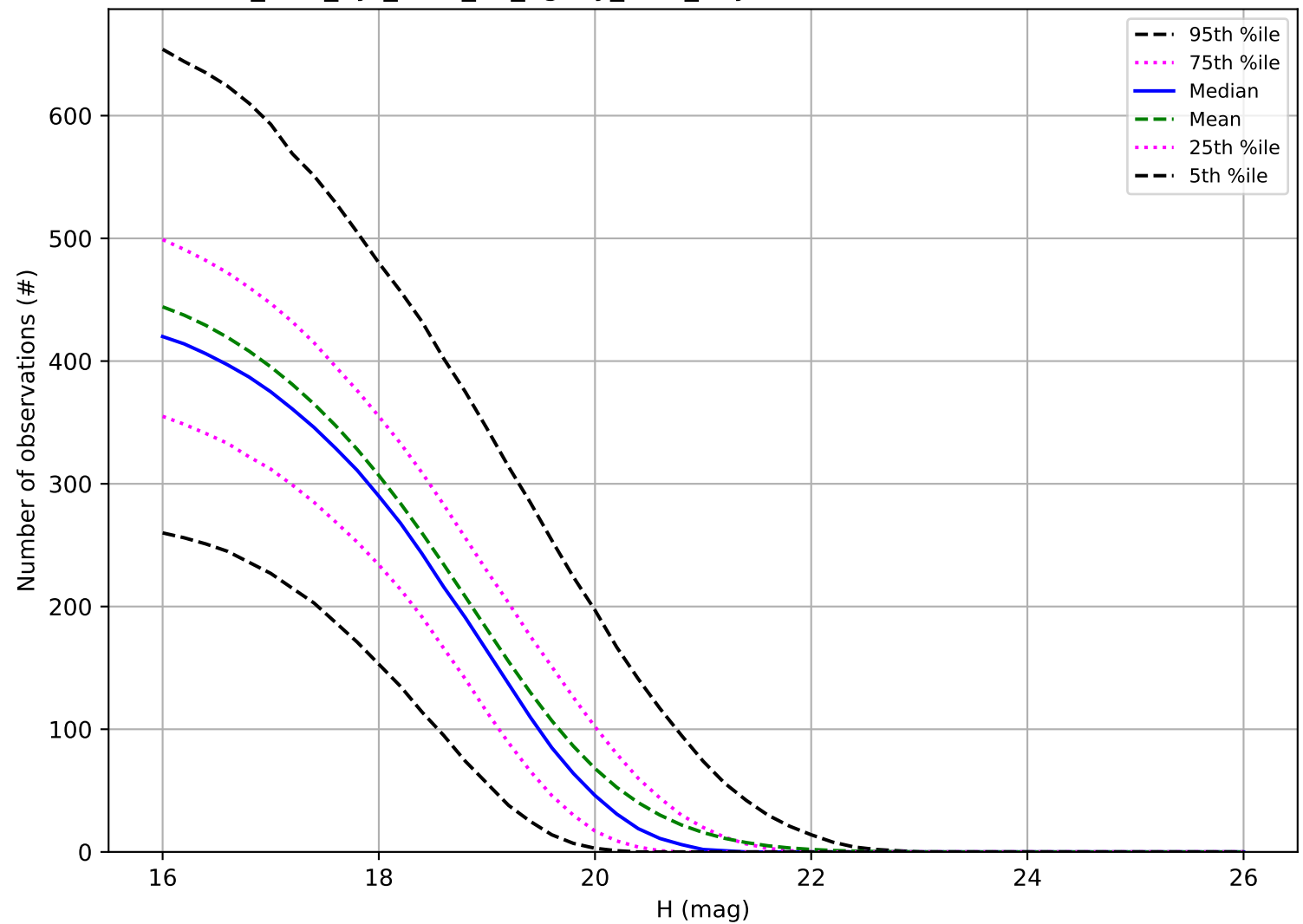
too_elab_2yr_r128_d2_ugrizy_v3.4_10yrs: Number of observations MBA
