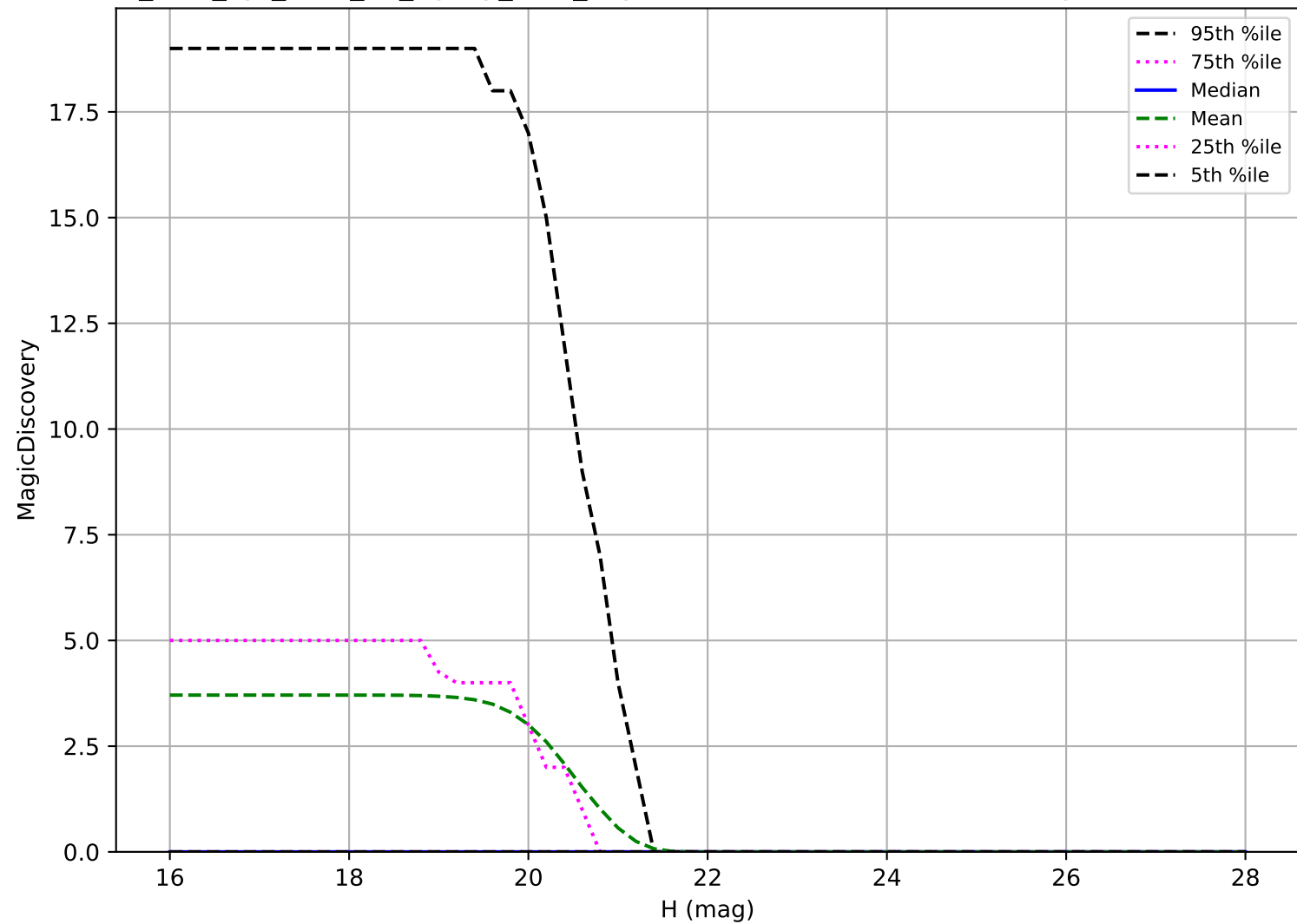
too_elab_2yr_r128_d2_ugrizy_v3.4_10yrs: Vatira 6 detections in 60 nights detection loss
