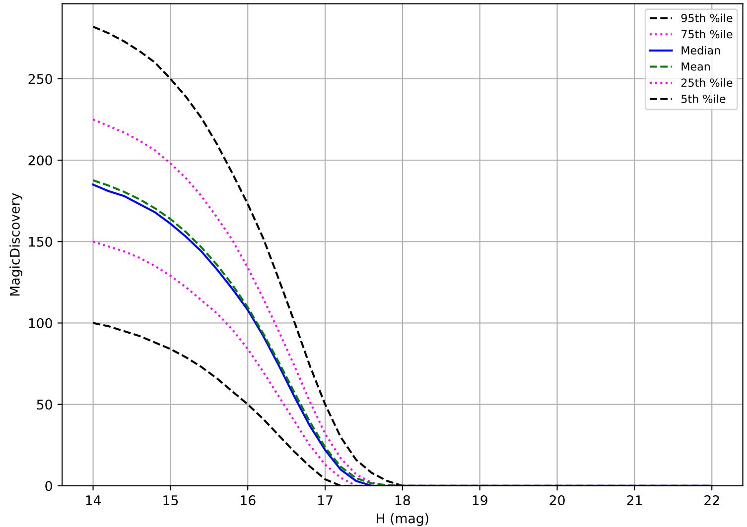
too_elab_2yr_r128_d2_ugrizy_v3.4_10yrs: Trojan 6 detections in 60 nights detection loss
