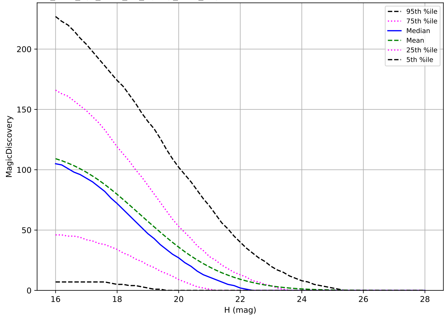
too_elab_2yr_r128_d2_ugrizy_v3.4_10yrs: PHA 6 detections in 60 nights detection loss
