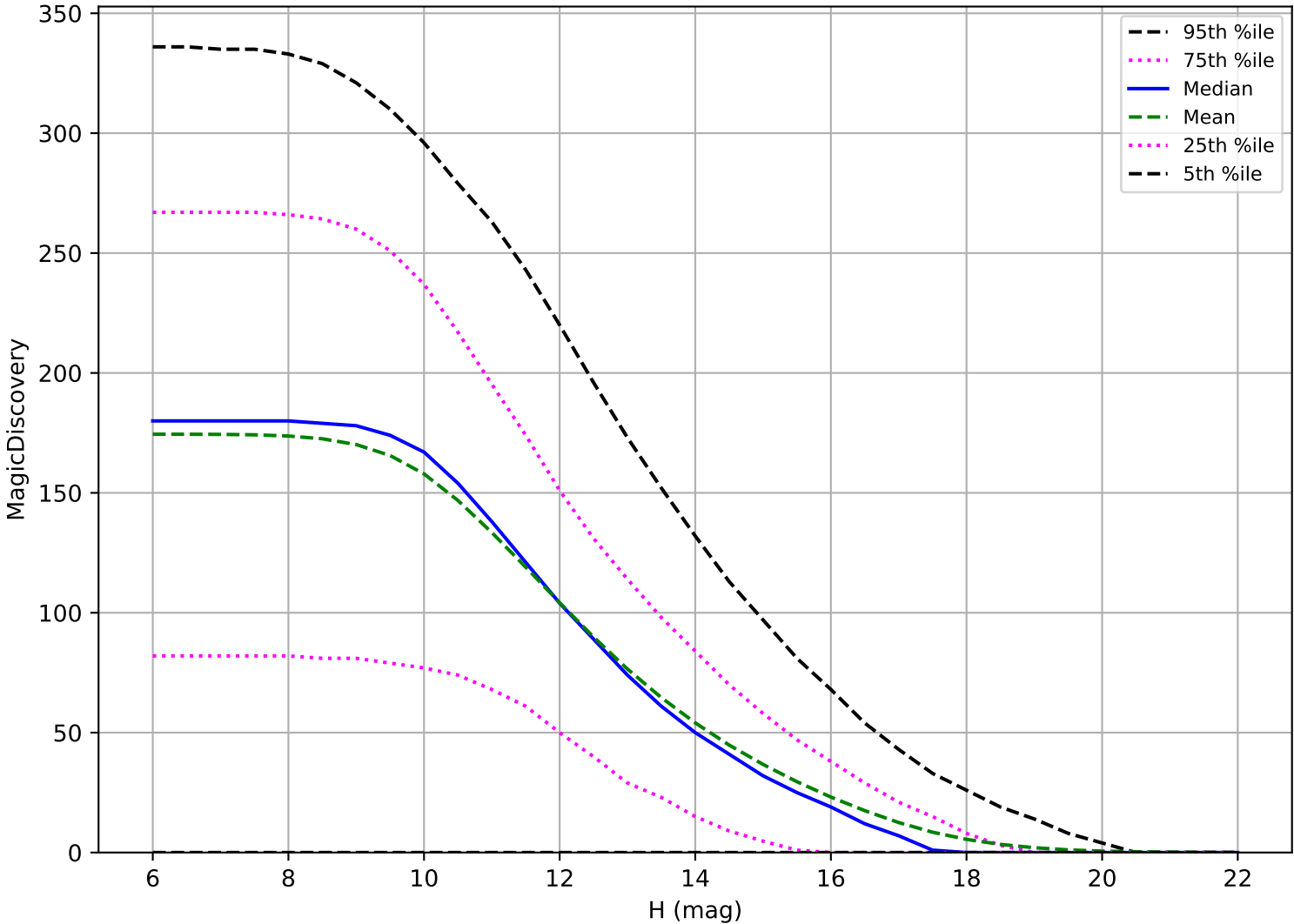
too_elab_2yr_r128_d2_ugrizy_v3.4_10yrs: OCC_r5 6 detections in 60 nights detection loss
