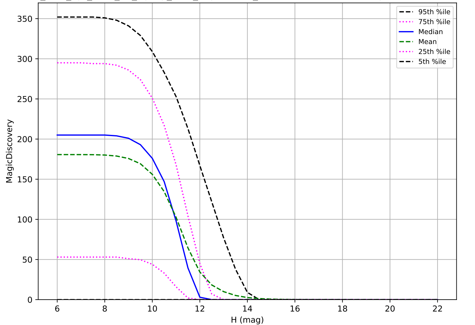
too_elab_2yr_r128_d2_ugrizy_v3.4_10yrs: OCC_r20 6 detections in 60 nights detection loss
