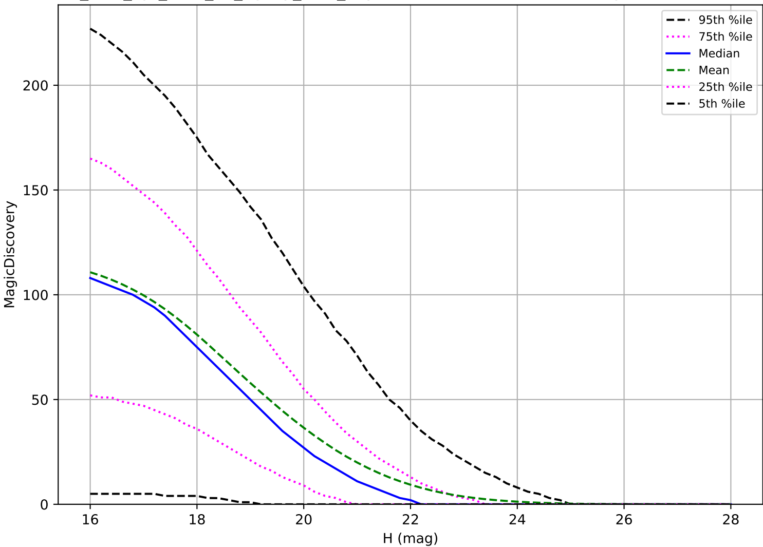
too_elab_2yr_r128_d2_ugrizy_v3.4_10yrs: NEO 6 detections in 60 nights detection loss
