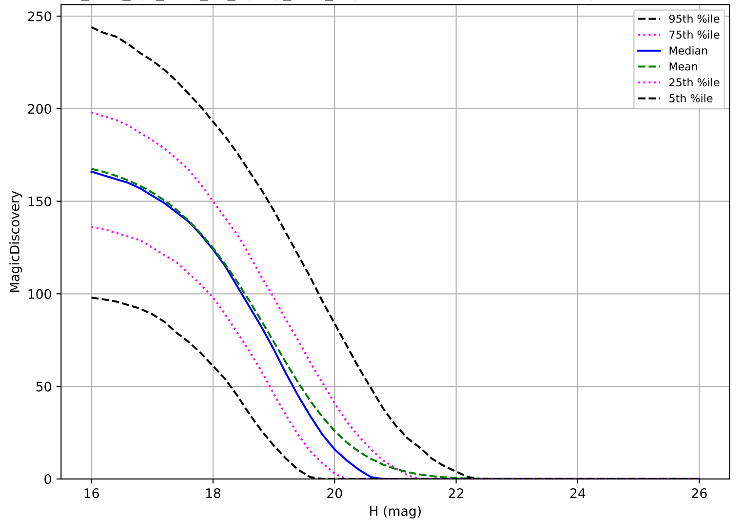
too_elab_2yr_r128_d2_ugrizy_v3.4_10yrs: MBA 6 detections in 60 nights detection loss
