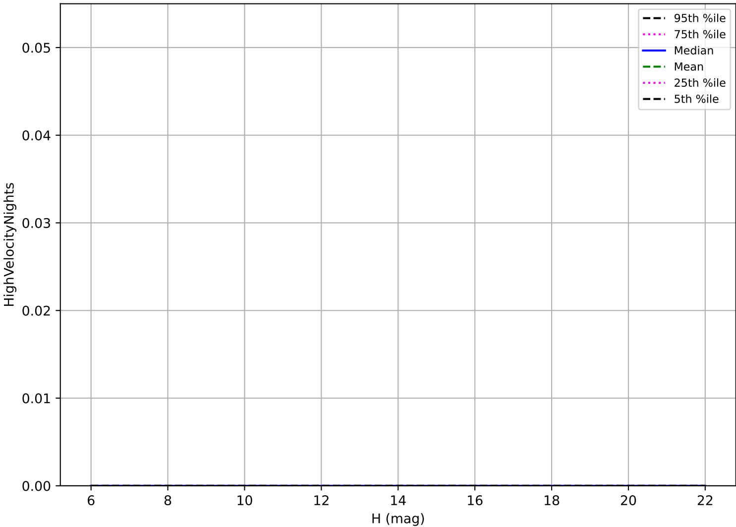
too_elab_2yr_r128_d2_ugrizy_v3.4_10yrs: OCC_r5 High velocity pair detection loss
