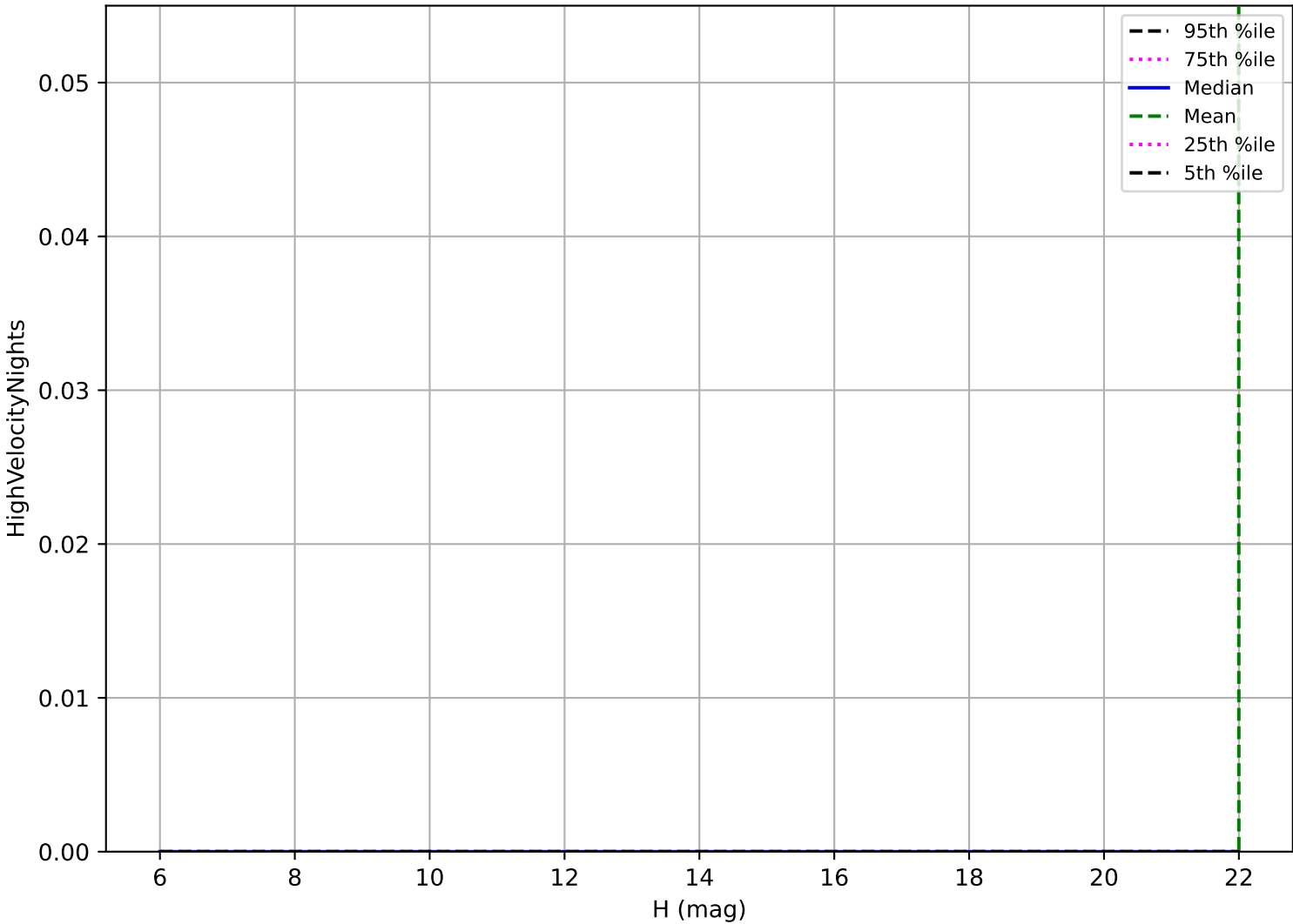
too_elab_2yr_r128_d2_ugrizy_v3.4_10yrs: OCC_r20 High velocity pair detection loss
