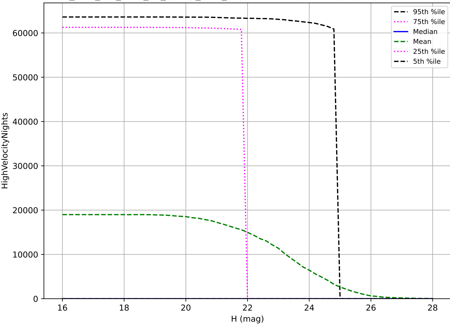
too_elab_2yr_r128_d2_ugrizy_v3.4_10yrs: NEO High velocity pair detection loss
