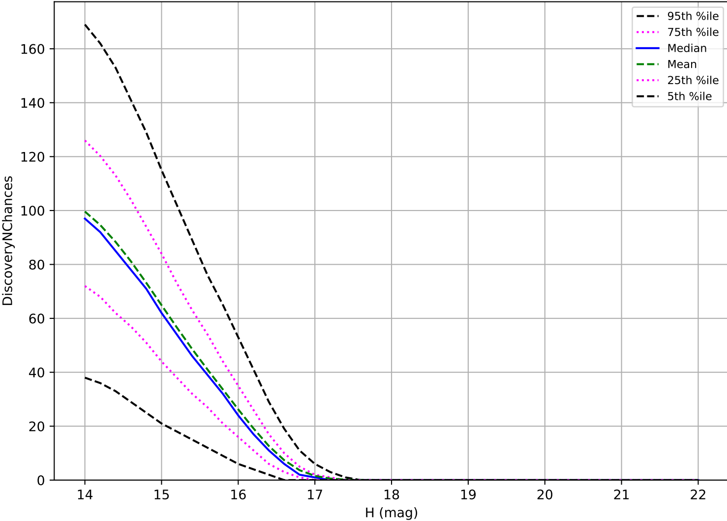
too_elab_2yr_r128_d2_ugrizy_v3.4_10yrs: Trojan 3 pairs in 15 nights detection loss
