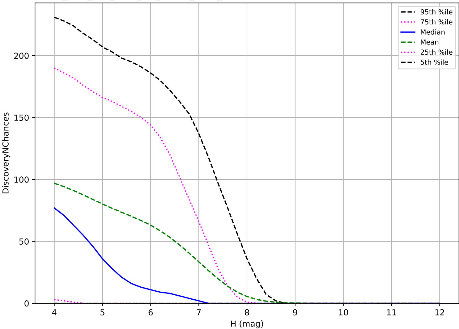
too_elab_2yr_r128_d2_ugrizy_v3.4_10yrs: TNO 3 pairs in 15 nights detection loss
