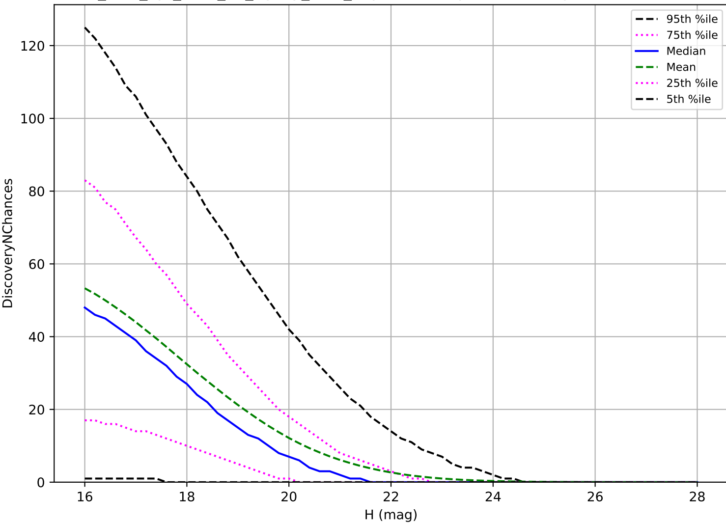
too_elab_2yr_r128_d2_ugrizy_v3.4_10yrs: PHA 3 pairs in 15 nights detection loss
