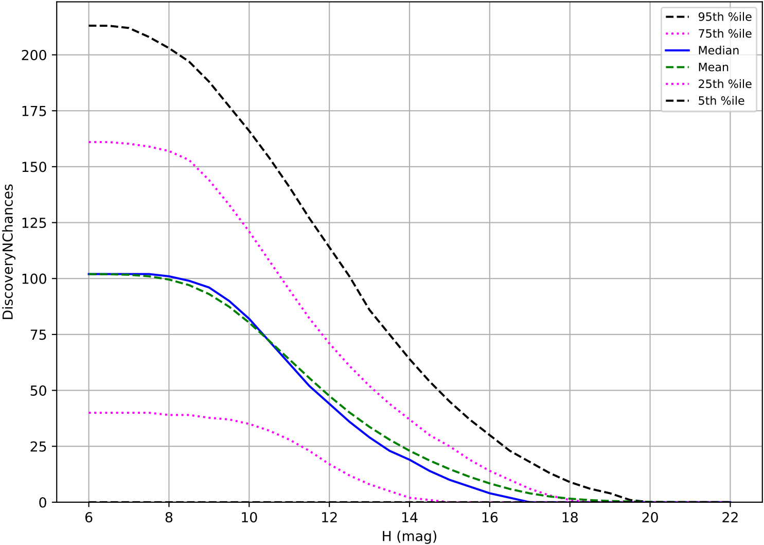
too_elab_2yr_r128_d2_ugrizy_v3.4_10yrs: OCC_r5 3 pairs in 15 nights detection loss
