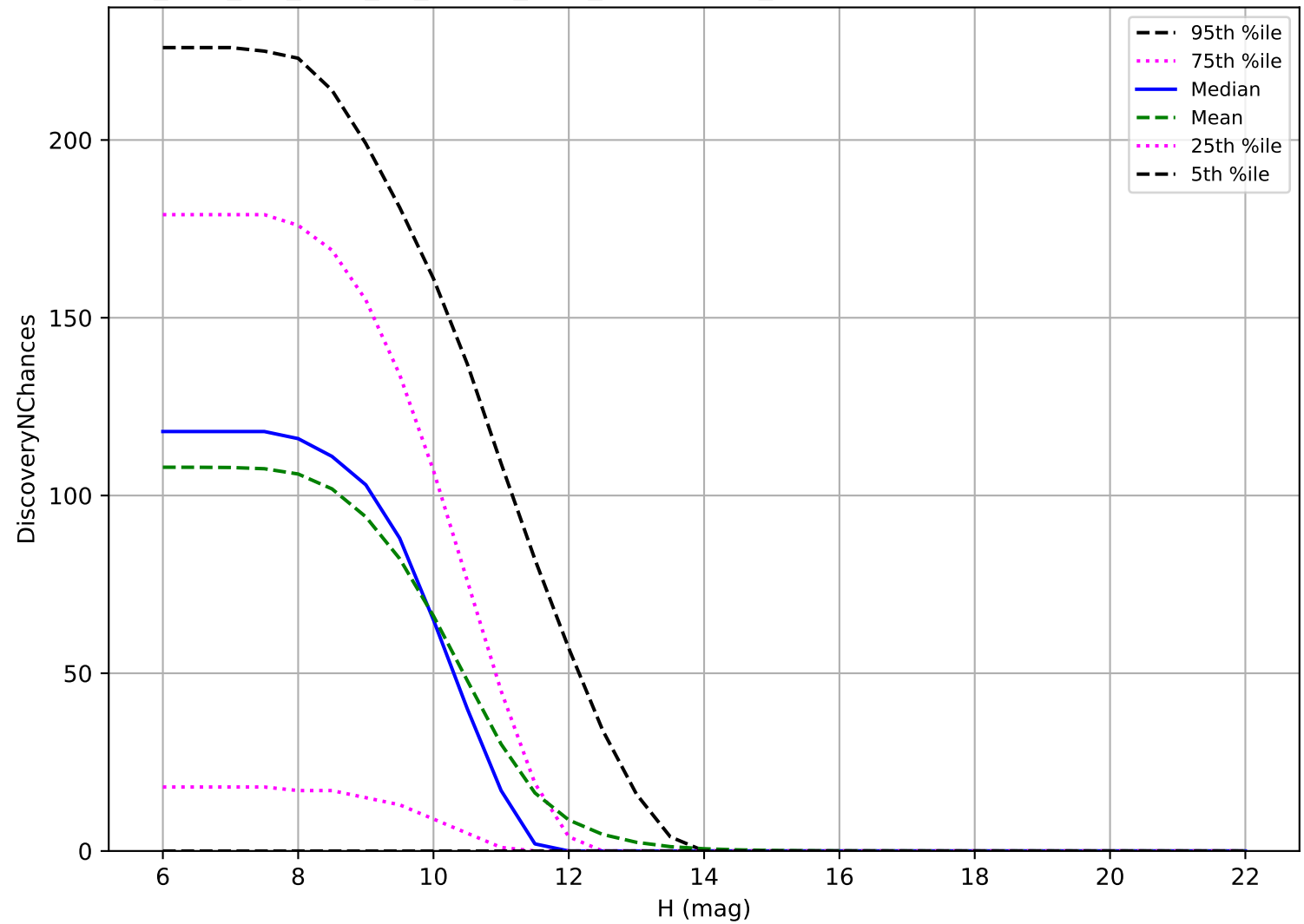
too_elab_2yr_r128_d2_ugrizy_v3.4_10yrs: OCC_r20 3 pairs in 15 nights detection loss
