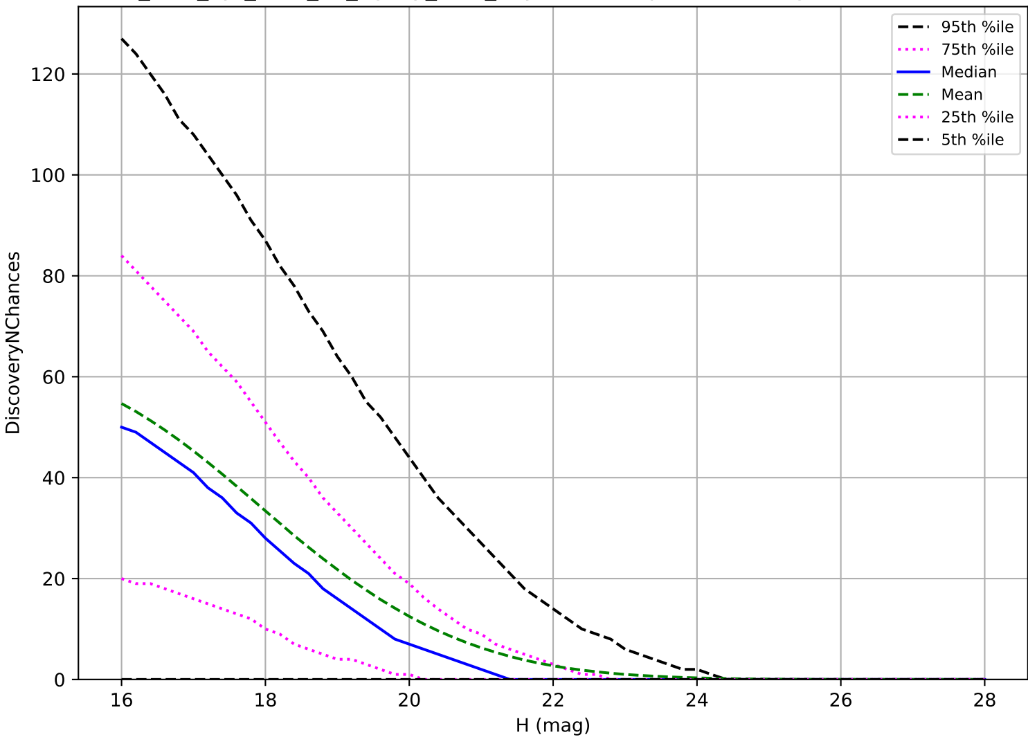
too_elab_2yr_r128_d2_ugrizy_v3.4_10yrs: NEO 3 pairs in 15 nights detection loss
