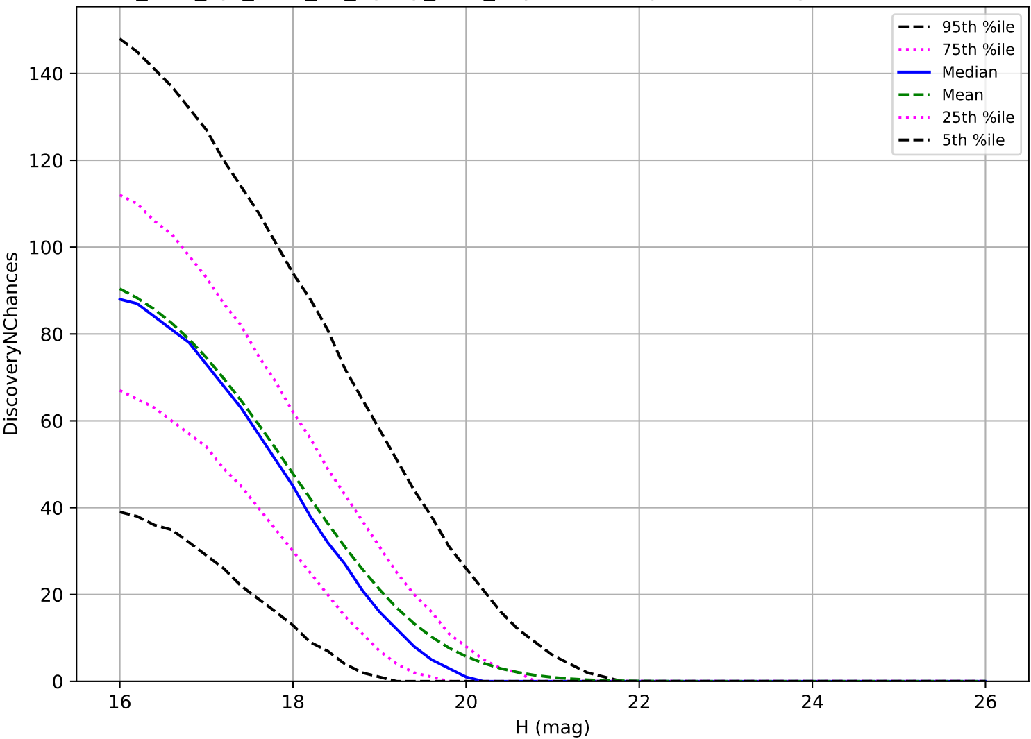
too_elab_2yr_r128_d2_ugrizy_v3.4_10yrs: MBA 3 pairs in 15 nights detection loss
