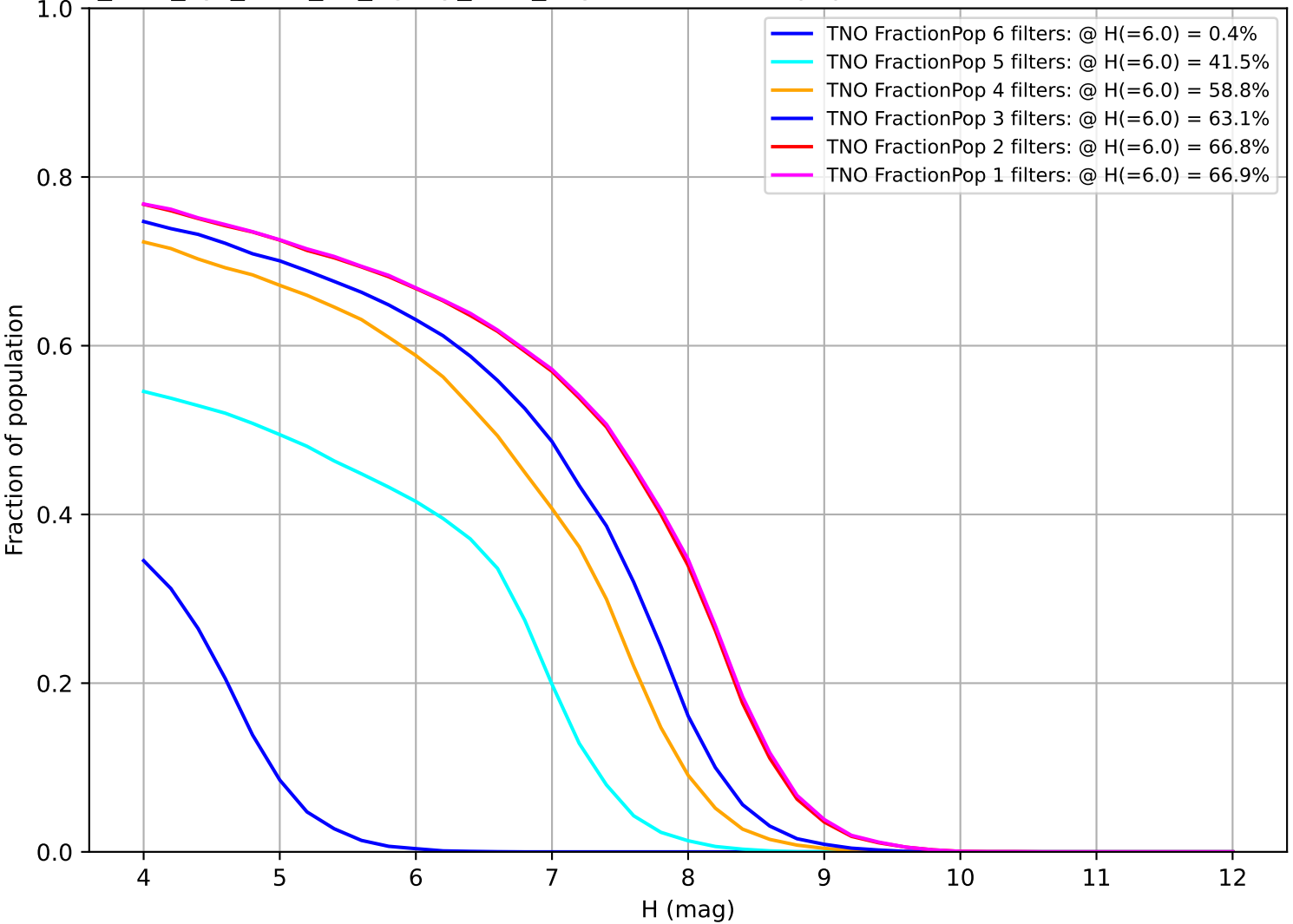
too_elab_2yr_r128_d2_ugrizy_v3.4_10yrs: Fraction of population with colors in X filters TNO
