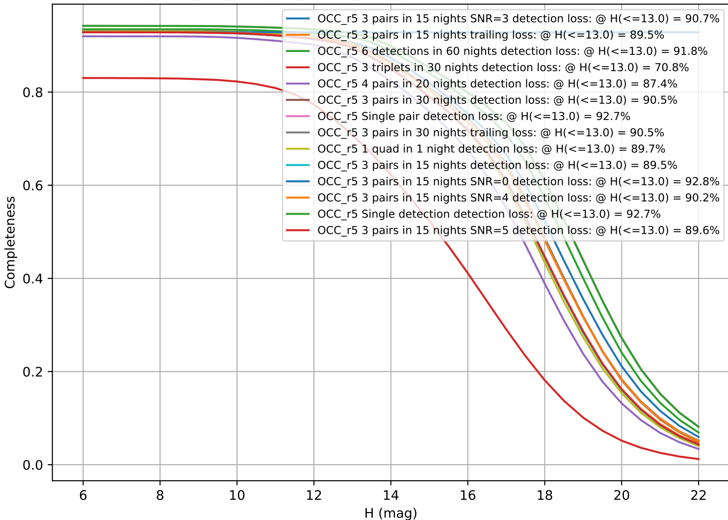
too_elab_2yr_r128_d2_ugrizy_v3.4_10yrs: CumulativeCompleteness
