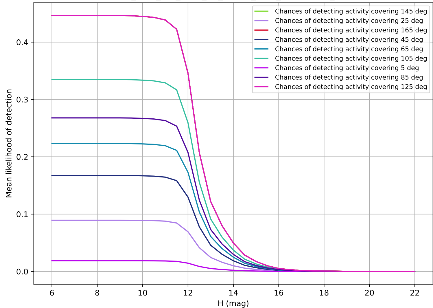
too_elab_2yr_r128_d2_ugrizy_v3.4_10yrs OCC_r20
