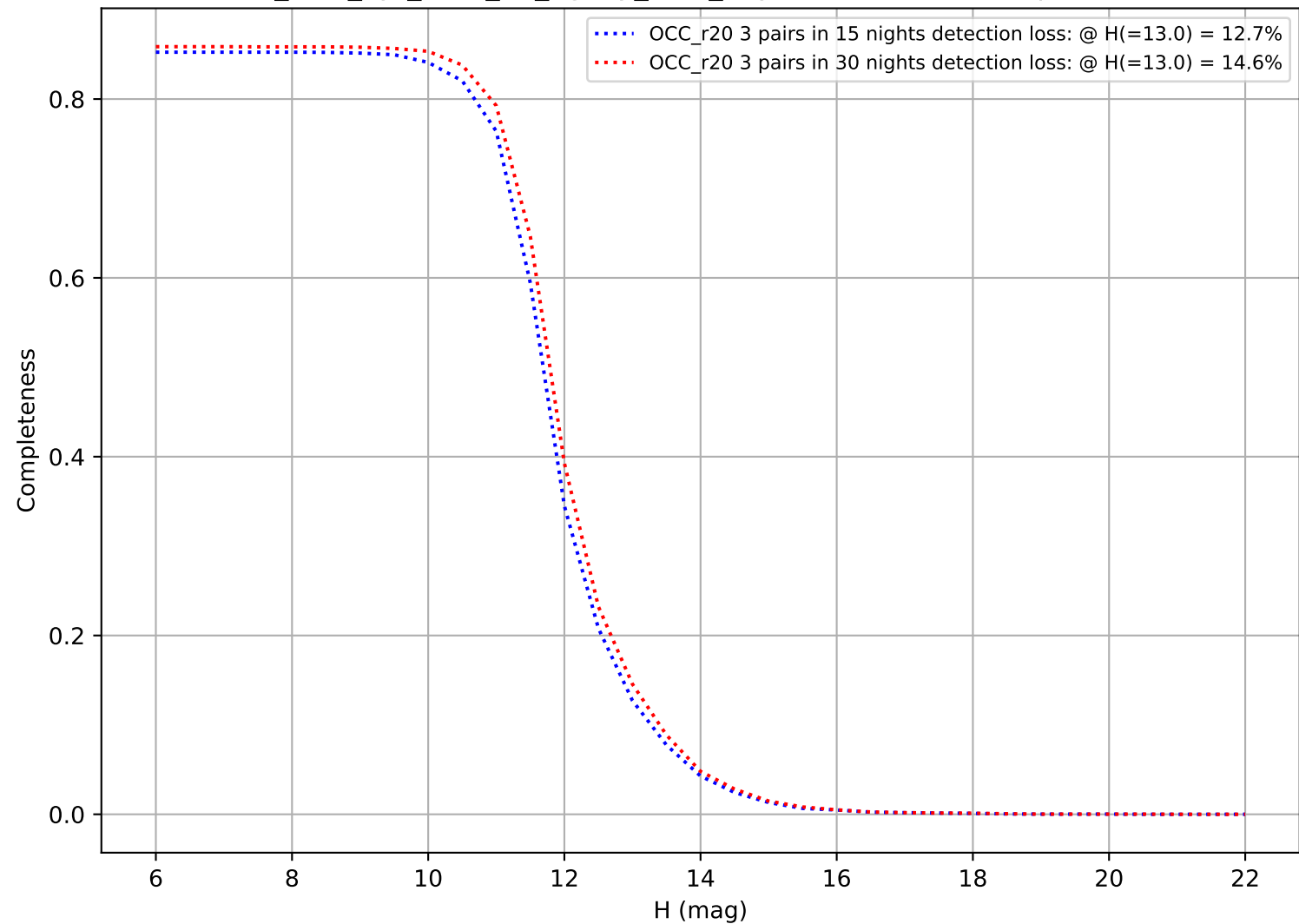
too_elab_2yr_r128_d2_ugrizy_v3.4_10yrs: DifferentialCompleteness
