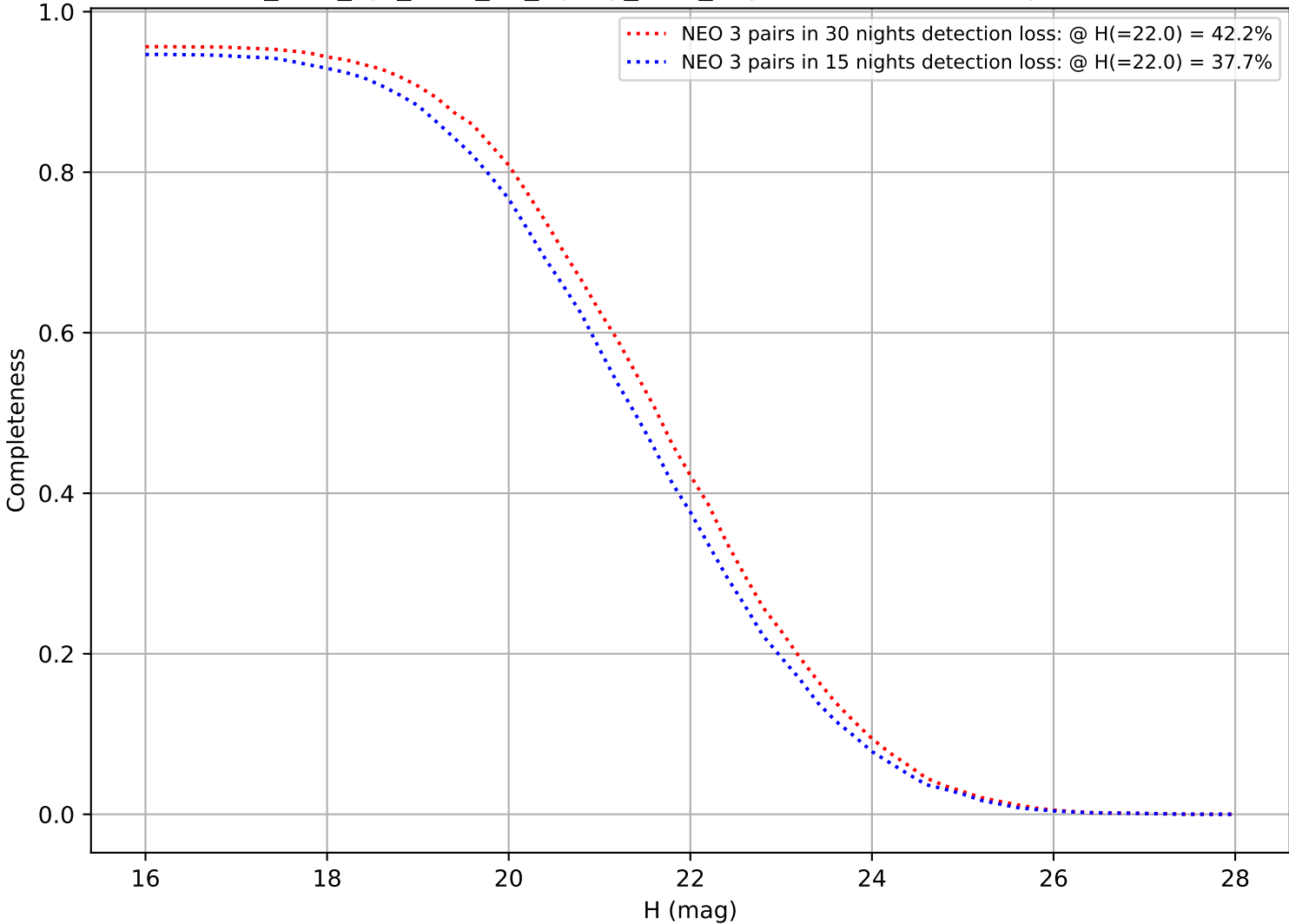
too_elab_2yr_r128_d2_ugrizy_v3.4_10yrs: DifferentialCompleteness
