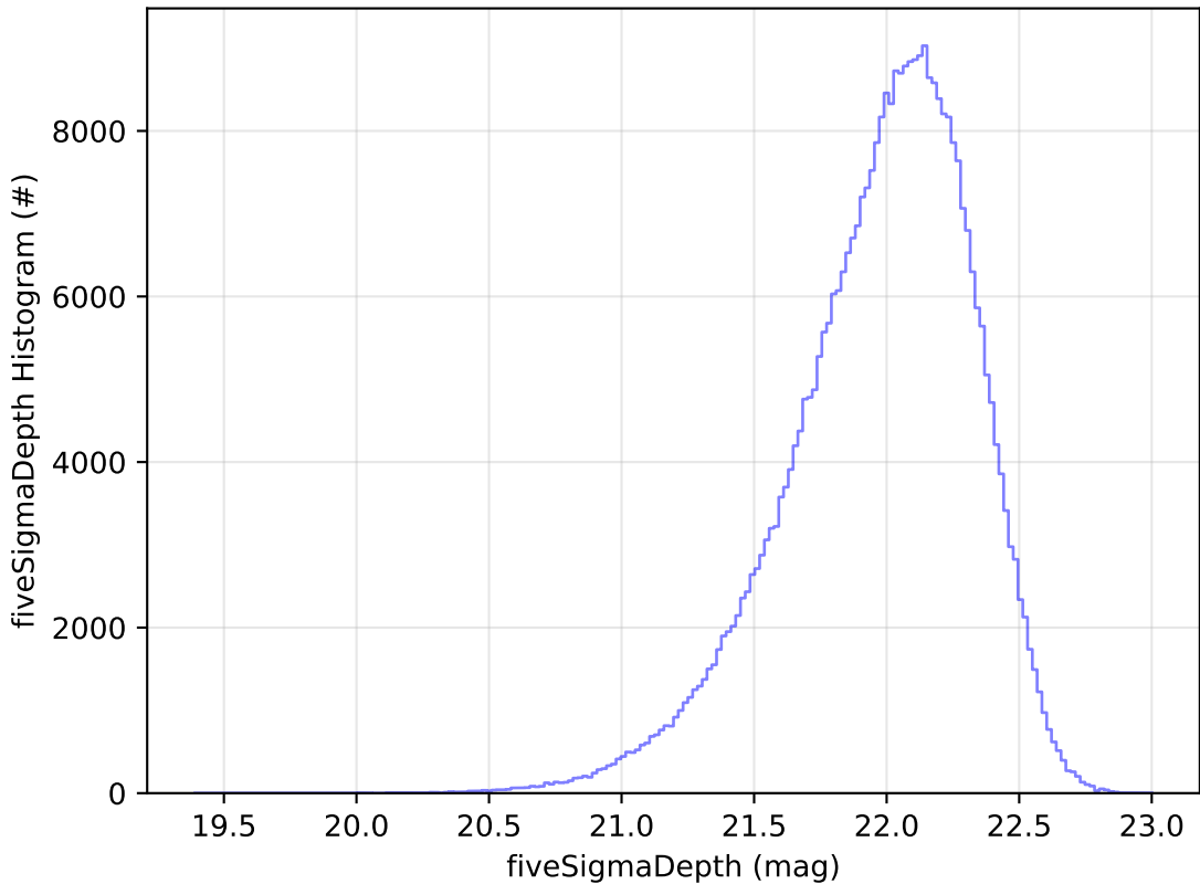
too_elab_2yr_r128_d2_ugrizy_v3.4_10yrs y: fiveSigmaDepth Histogram
