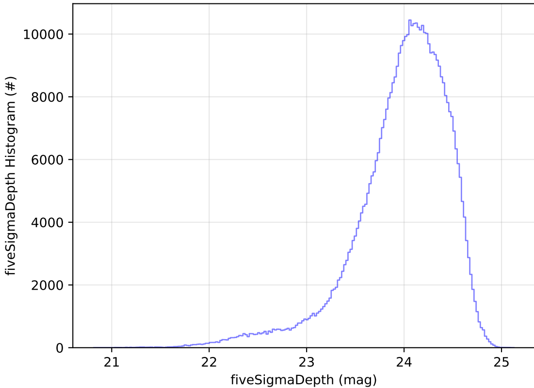
too_elab_2yr_r128_d2_ugrizy_v3.4_10yrs r: fiveSigmaDepth Histogram
