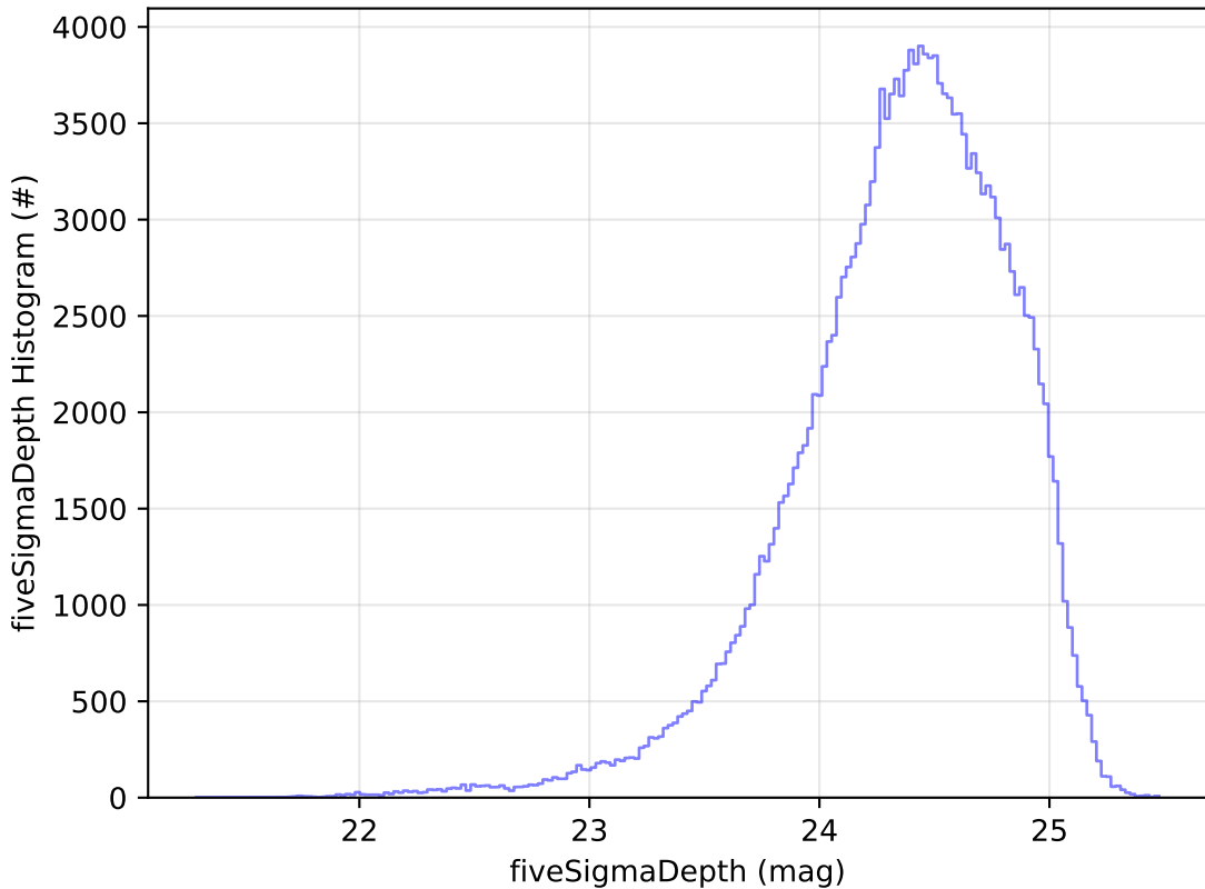
too_elab_2yr_r128_d2_ugrizy_v3.4_10yrs g: fiveSigmaDepth Histogram
