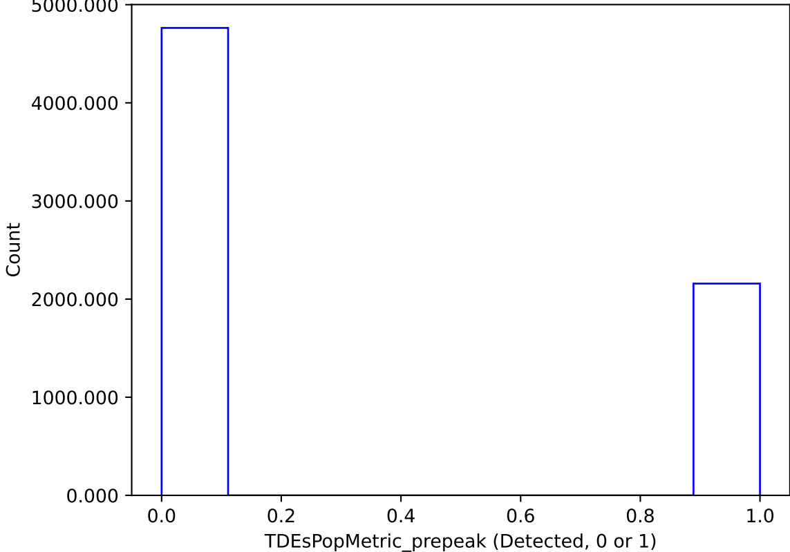
too_elab_2yr_r128_d2_ugrizy_v3.4_10yrs : TDEsPopMetric_prepeak
