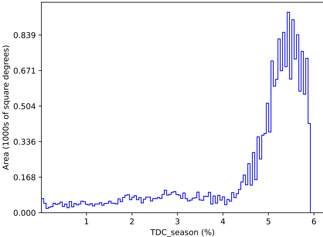
too_elab_2yr_r128_d2_ugrizy_v3.4_10yrs : TDC_season
