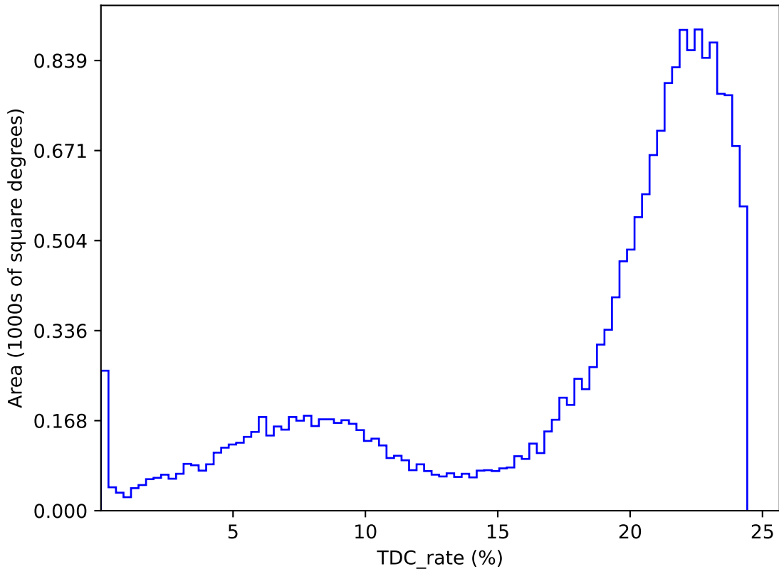
too_elab_2yr_r128_d2_ugrizy_v3.4_10yrs : TDC_rate
