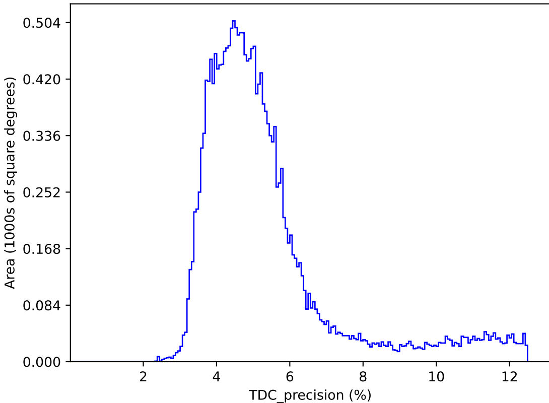
too_elab_2yr_r128_d2_ugrizy_v3.4_10yrs : TDC_precision
