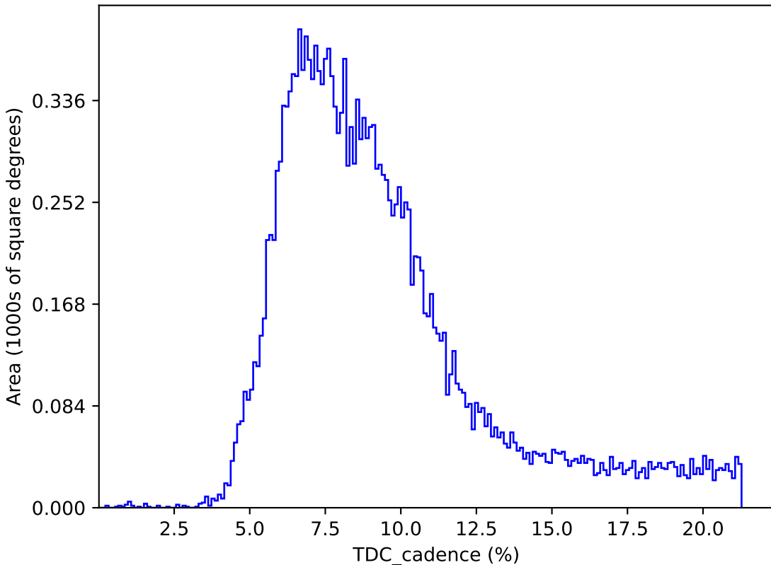
too_elab_2yr_r128_d2_ugrizy_v3.4_10yrs : TDC_cadence
