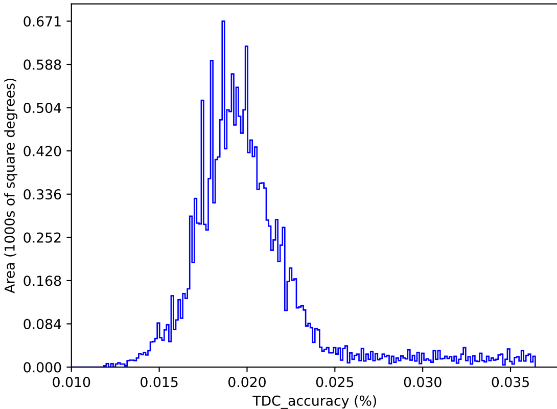
too_elab_2yr_r128_d2_ugrizy_v3.4_10yrs : TDC_accuracy
